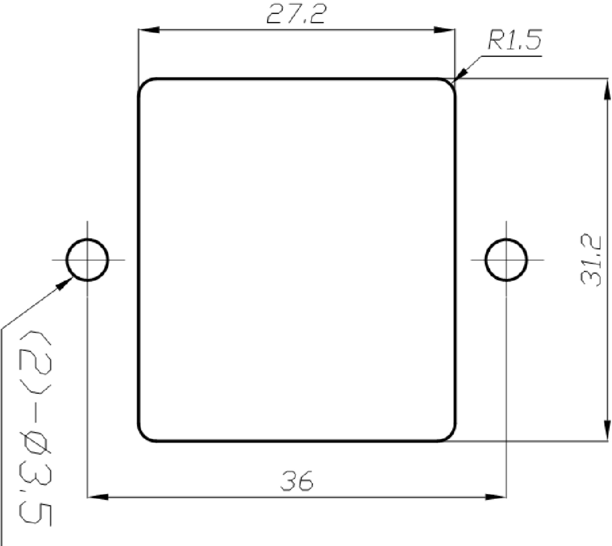
PANEL CUT-OUT
